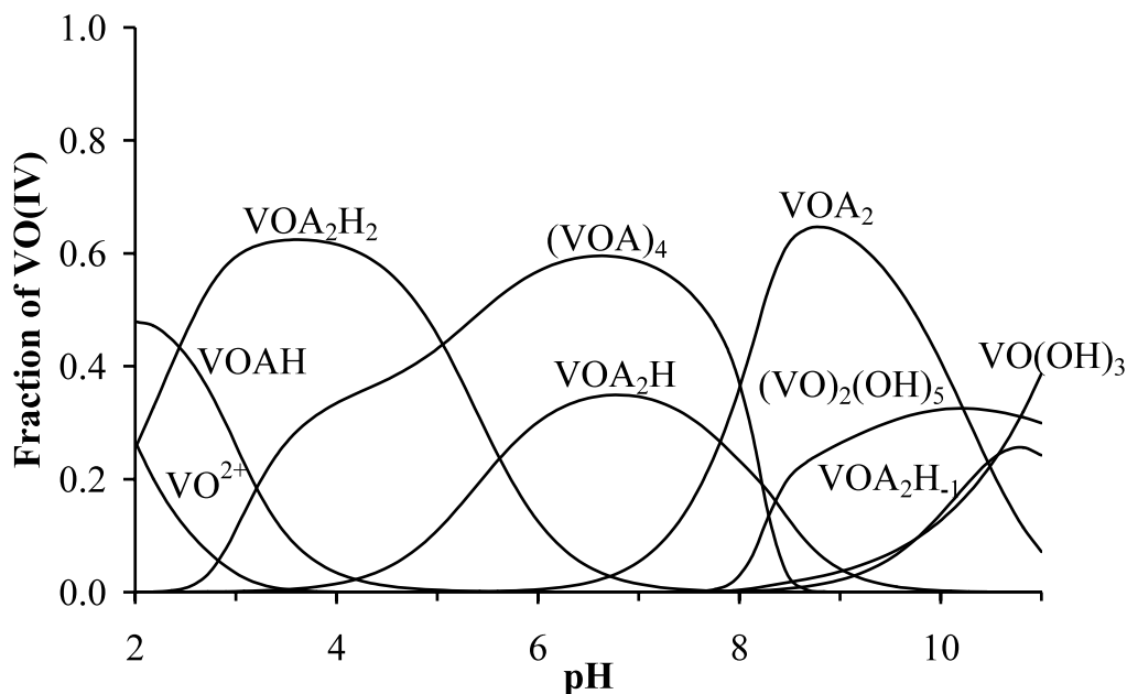
Fig. 1. Speciation curves for the complexes formed in the VO(IV)–3HPA system at 1:2 metal ion to ligand ratio, c_{\text{VO(IV)}} = 0.001 \text{ mol dm}^{-3} .
